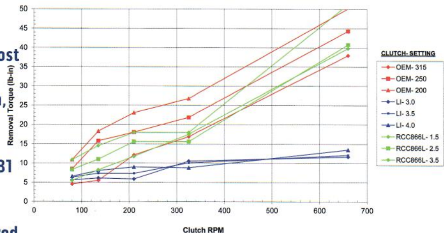
OEM versus RIMTEC LOW INERTIA CLUTCH Cap Removal Torques (Target is under 15 lb-in at 545 rpm)
